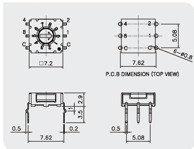
Crimped Type Layout
