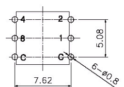
P.C.B DIMENSION (TOP VIEW)
