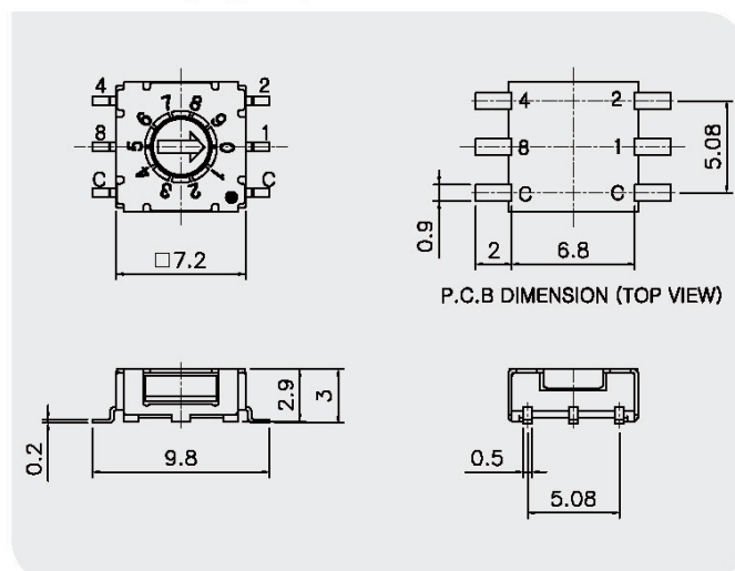
SMD Gull wing Type Layout
