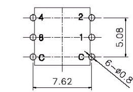
P.C.B DIMENSION (TOP VIEW)
