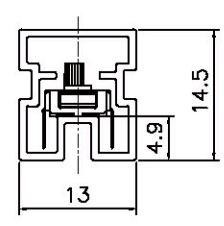
M Type Actuator (Height : 3mm)
